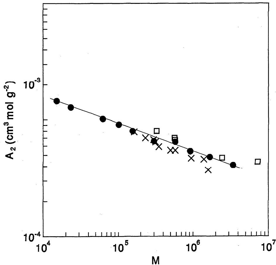
FIG. 2. A_2 as a function of M for 1,4-polyisoprene in cyclohexane (● = Ref. 31 via low angle light scattering; x = Ref. 31 via multi-angle light scattering; □ = data from other sources).
